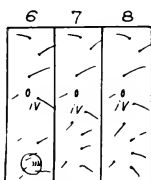
Fig. 482. Setal map of 6th, 7th and 8th abdominal segments.
